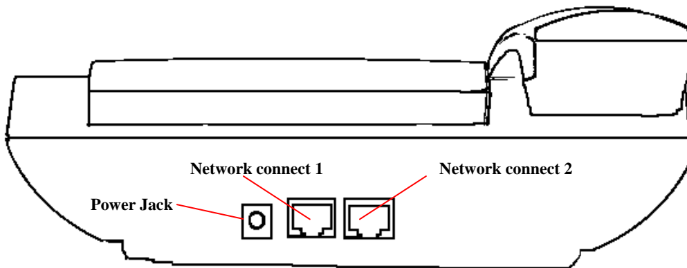
Fig 4.1.2 GP1266 IAX2 Phone Back
